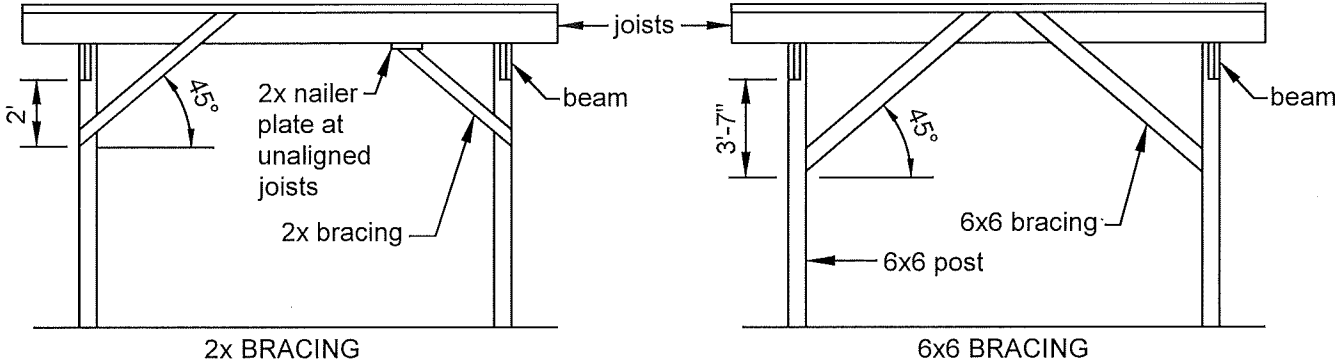
FIGURE 23: DIAGONAL BRACING AT BEAM-POST LOCATIONS
