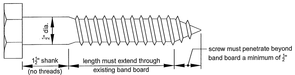
FIGURE 17: LAG SCREW
