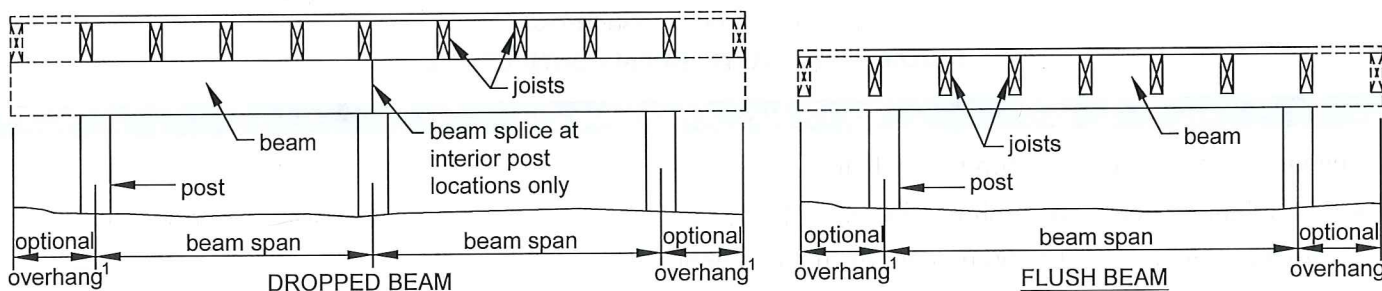
FIGURE 5: BEAM TYPES
