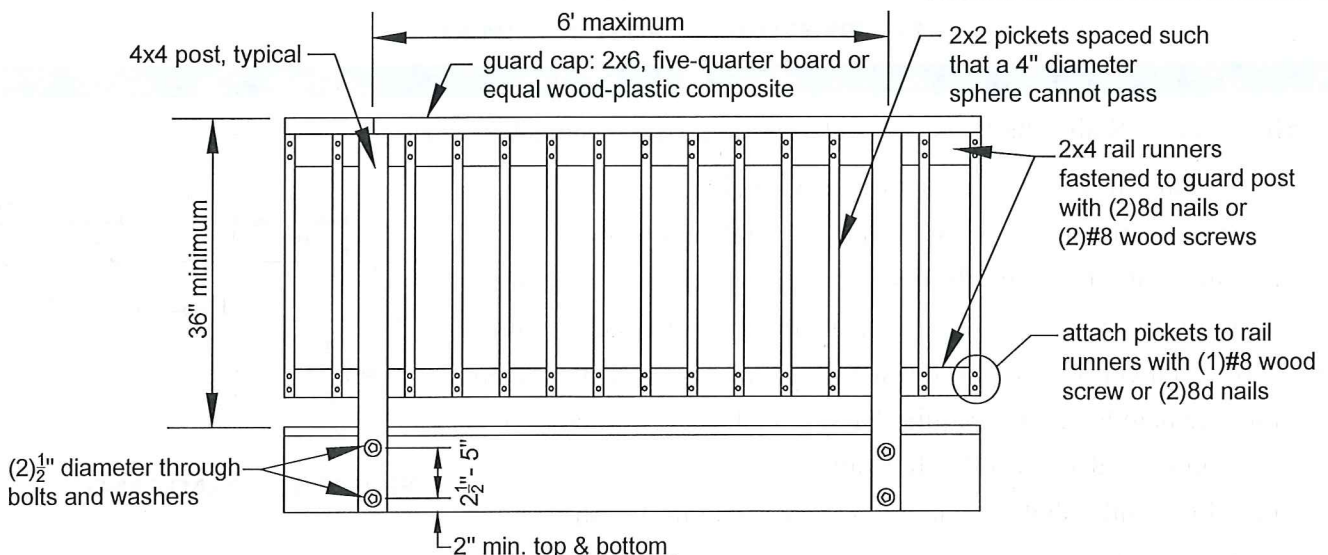
FIGURE 29: GUARDS
