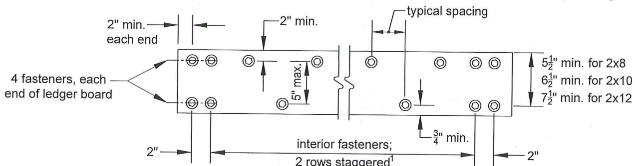
FIGURE 16: LEDGER BOARD FASTENER SPACING AND CLEARANCES
