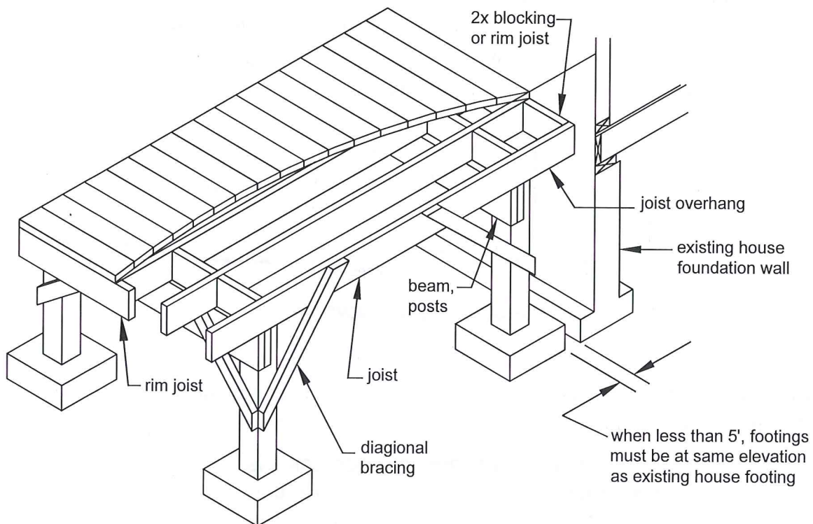
FIGURE 19: FREE-STANDING DECK
