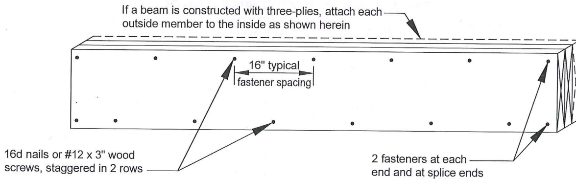
FIGURE 6: BEAM ASSEMBLY
