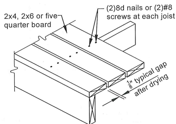
FIGURE 1: TYPICAL DECKING
