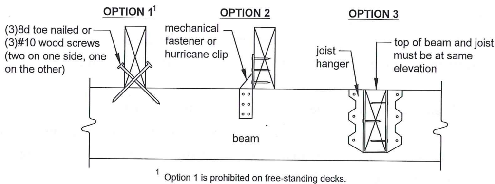
FIGURE 7: JOIST-TO-BEAM CONNECTION
