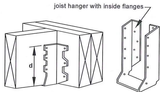
FIGURE 8: JOIST HANGERS
