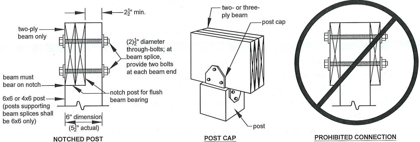
FIGURE 9: POST-TO-BEAM CONNECTIONS
