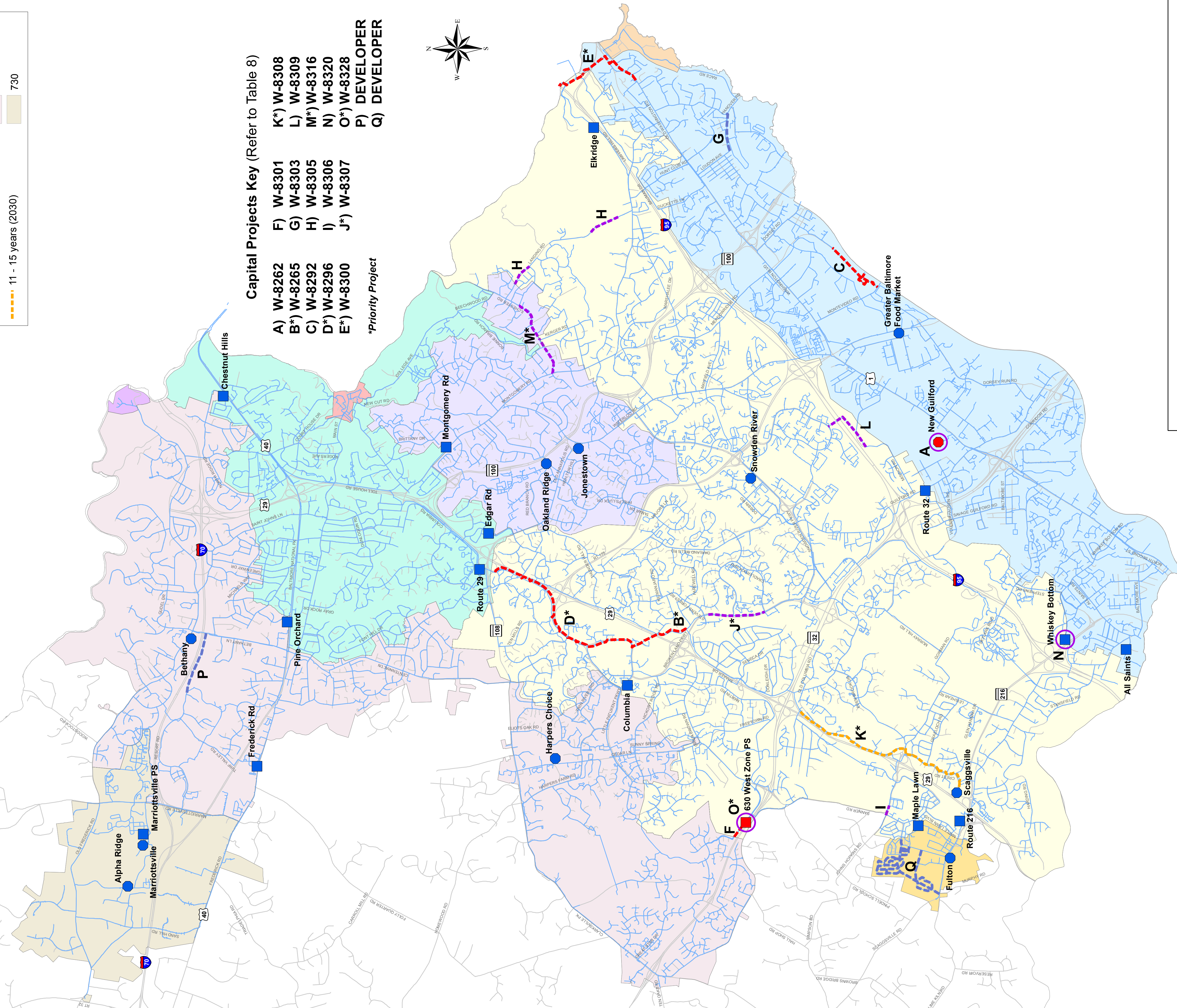
FIGURE 3-4 Immediate, 5-Year, 10-Year and Comprehensive Priorities Plan for Water System Development November 2015
