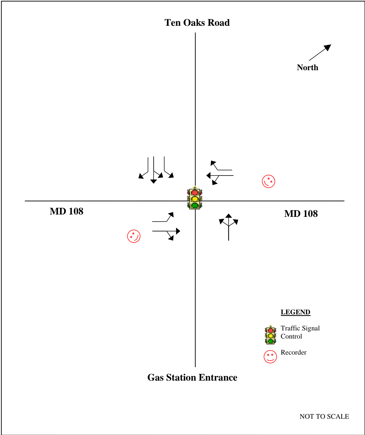
Figure 1. Lane Configuration: MD 108 at Ten Oaks Road / Gas Station Entrance Howard County, MD
