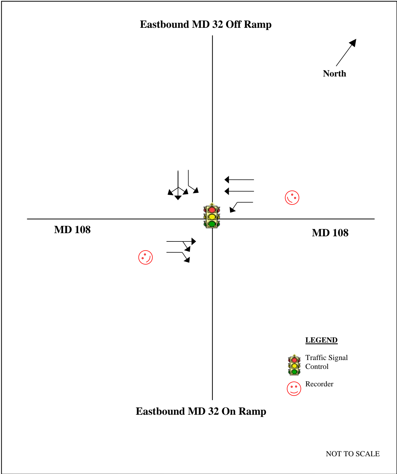
Figure 1. Lane Configuration: MD 108 at MD 32 Eastbound Ramps Howard County, MD
