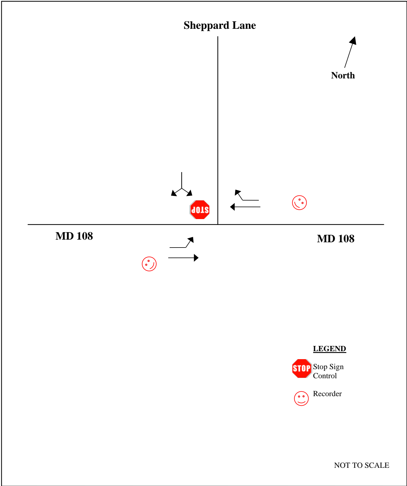
Figure 1. Lane Configuration: MD 108 at Sheppard Lane Howard County, MD
