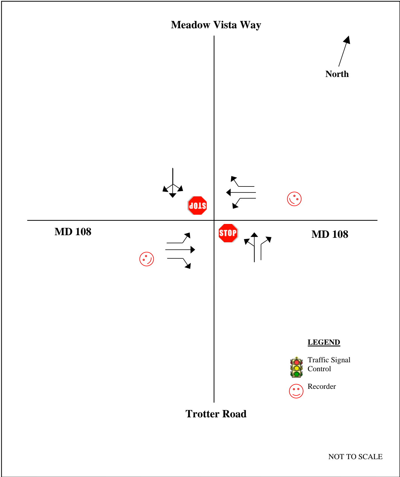
Figure 1. Lane Configuration: MD 108 at Meadow Vista Way / Trotter Road Howard County, MD
