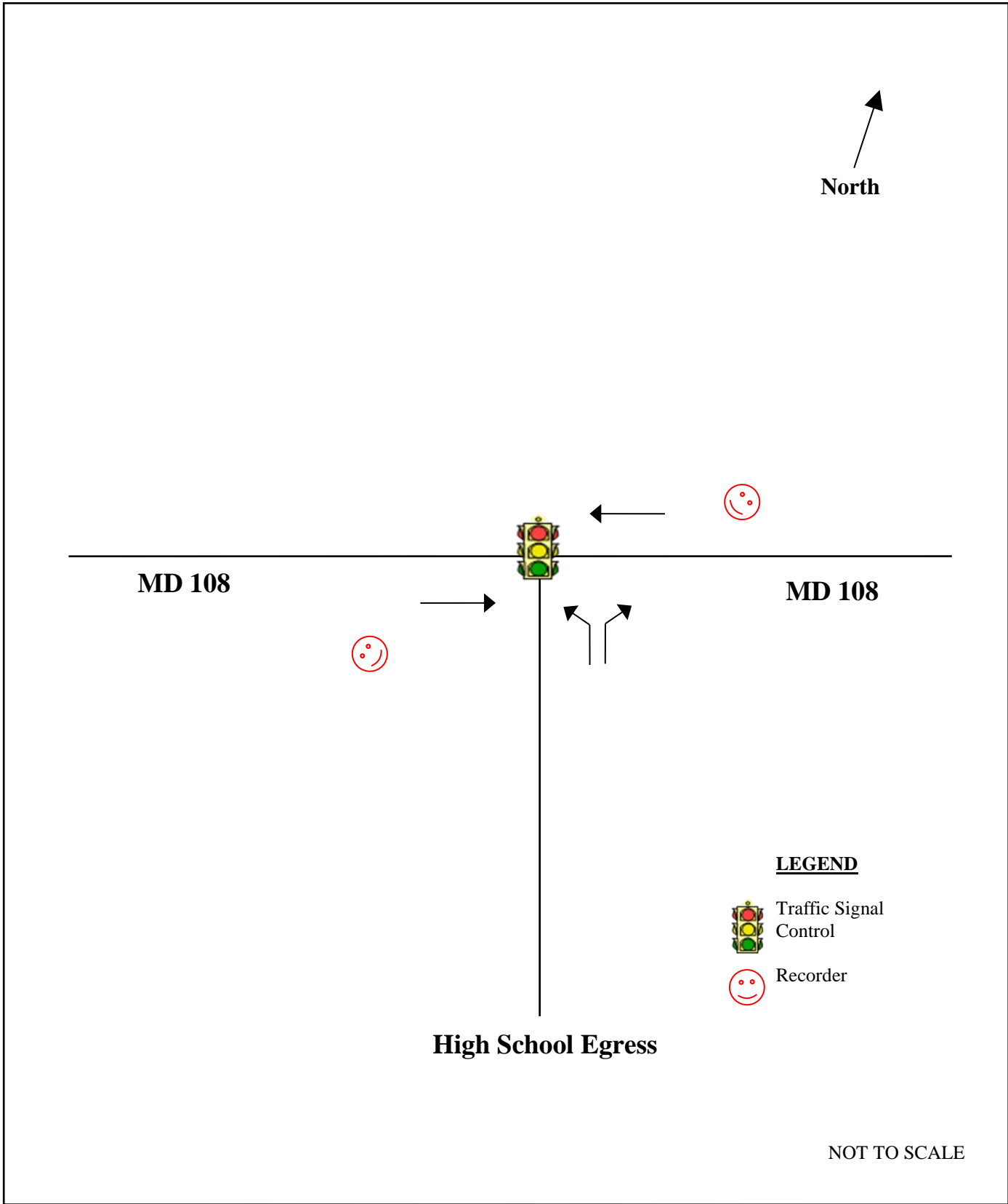
Figure 1. Lane Configuration: MD 108 at High School Egress Howard County, MD
