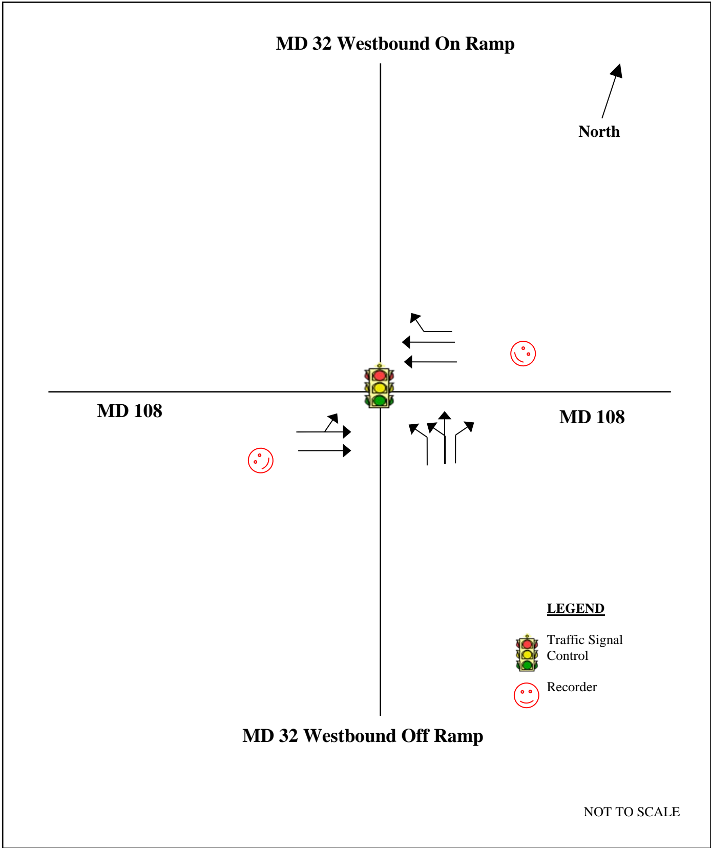
Figure 1. Lane Configuration: MD 108 at MD 32 Westbound Ramps Howard County, MD
