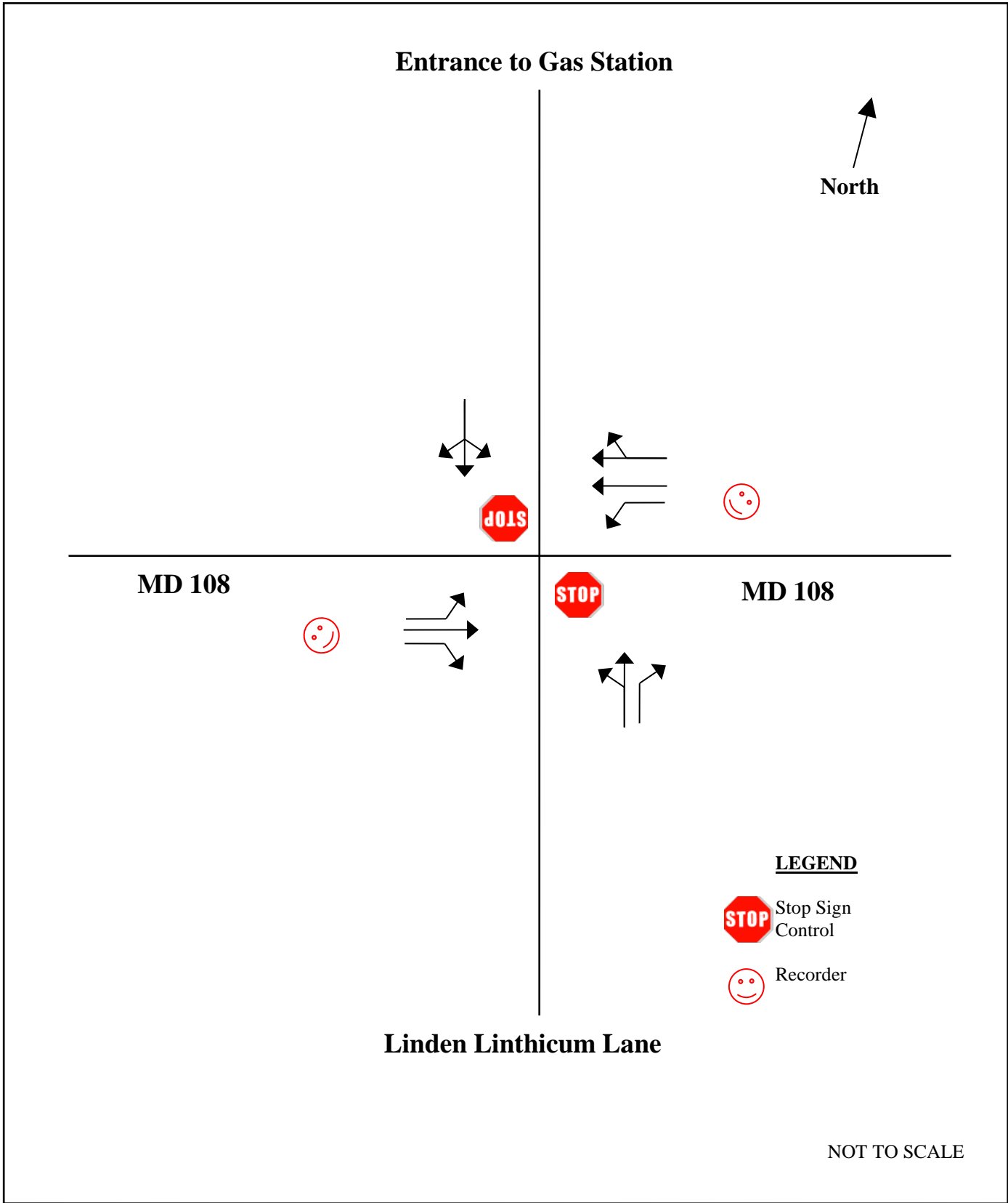
Figure 1. Lane Configuration: MD 108 at Linden Linthicum Lane Howard County, MD
